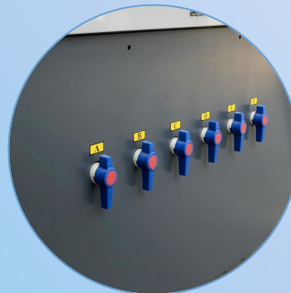
6 Zones Separated Vaccum Controller
