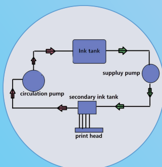
White Ink Circulation (With Stirring Function )
