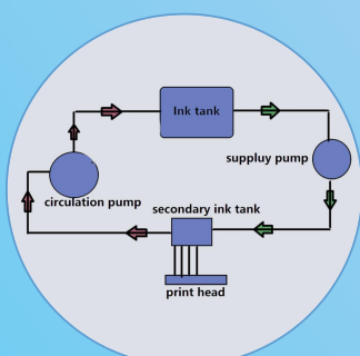
White Ink Circulation (With Stirring Function)
